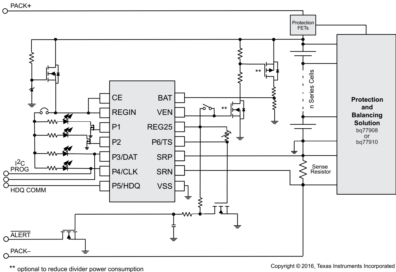
Figure 14. bq34z100-G1 Simplified Implementation
