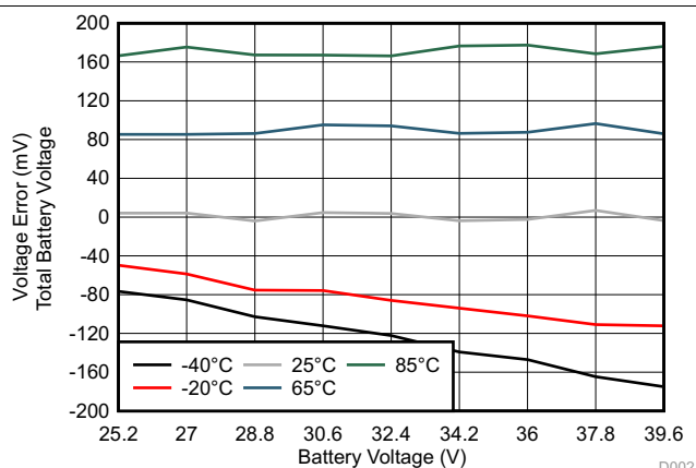
Figure 19. V_{\text{Err}} Across VIN (0 mA) 9 s
