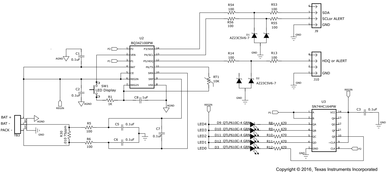
Figure 15. 1-Cell Li-Ion and 5-LED Display
