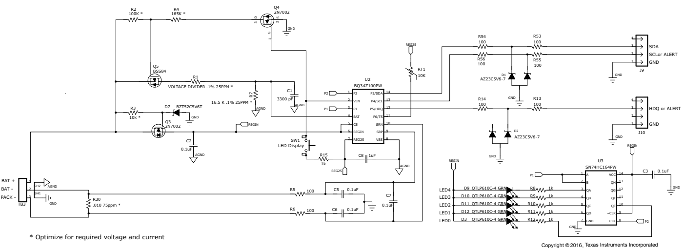
Figure 16. Multi-Cell and 5-LED Display
